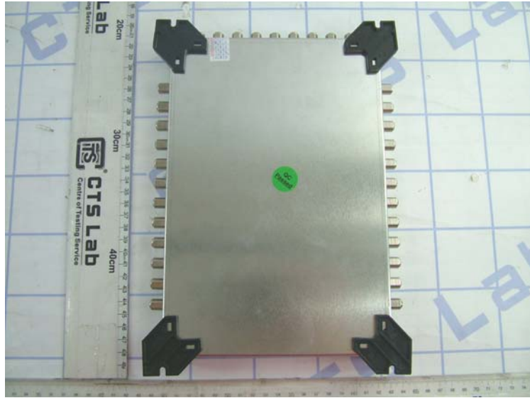
Figure 5 (External view-base)
