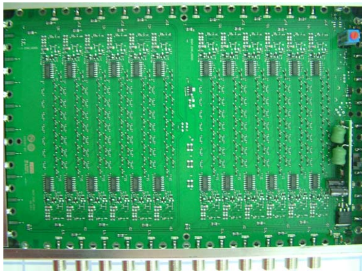
Figure 8 (PCB -side 1)
