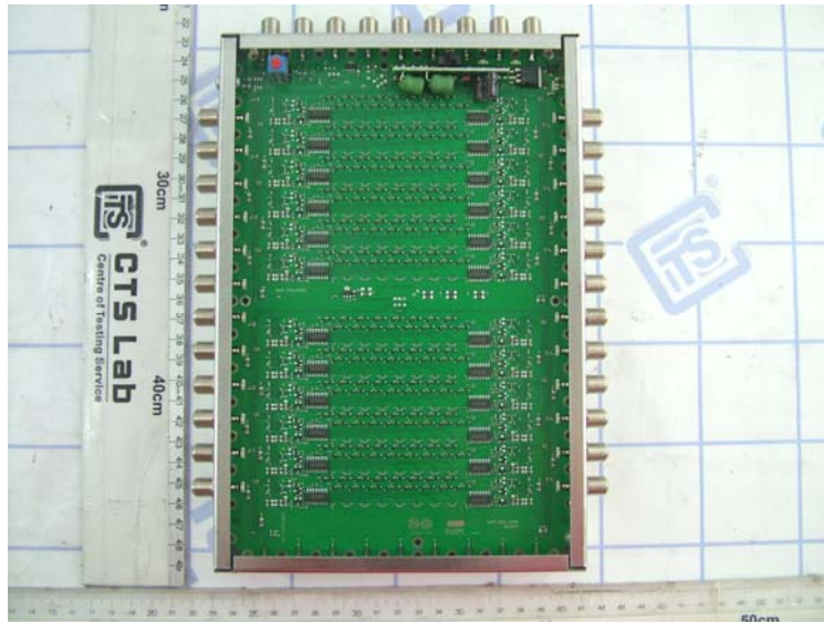
Figure 7 (Internal view -2)
